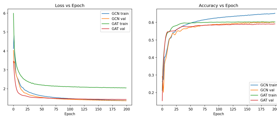
Figure 4 — Training Curves, file: training_curves.png
