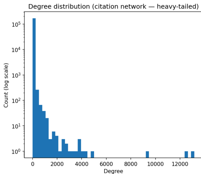
Figure 3 — Degree Distribution, file: degree_distribution.png
