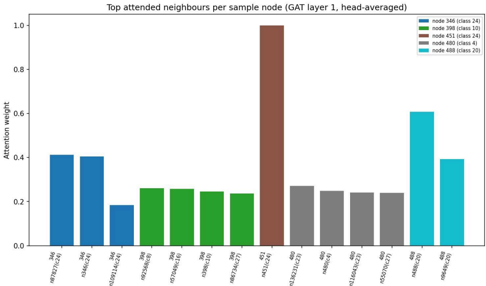
Figure 6 — GAT Attention-Weight Analysis, file: attention_analysis_chart.png
