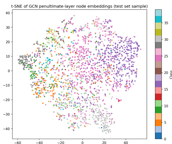
Figure 5 — Node Embedding Visualisation (t-SNE), file: embedding_tsne.png
